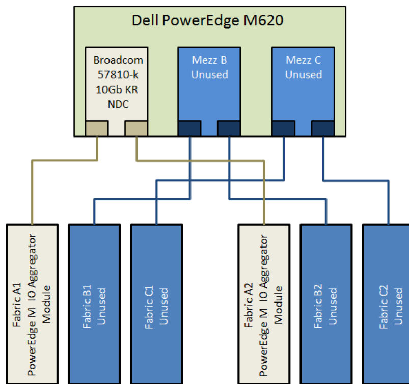
Figure 3: I/O Connectivity for PowerEdge M620 Blade Server
