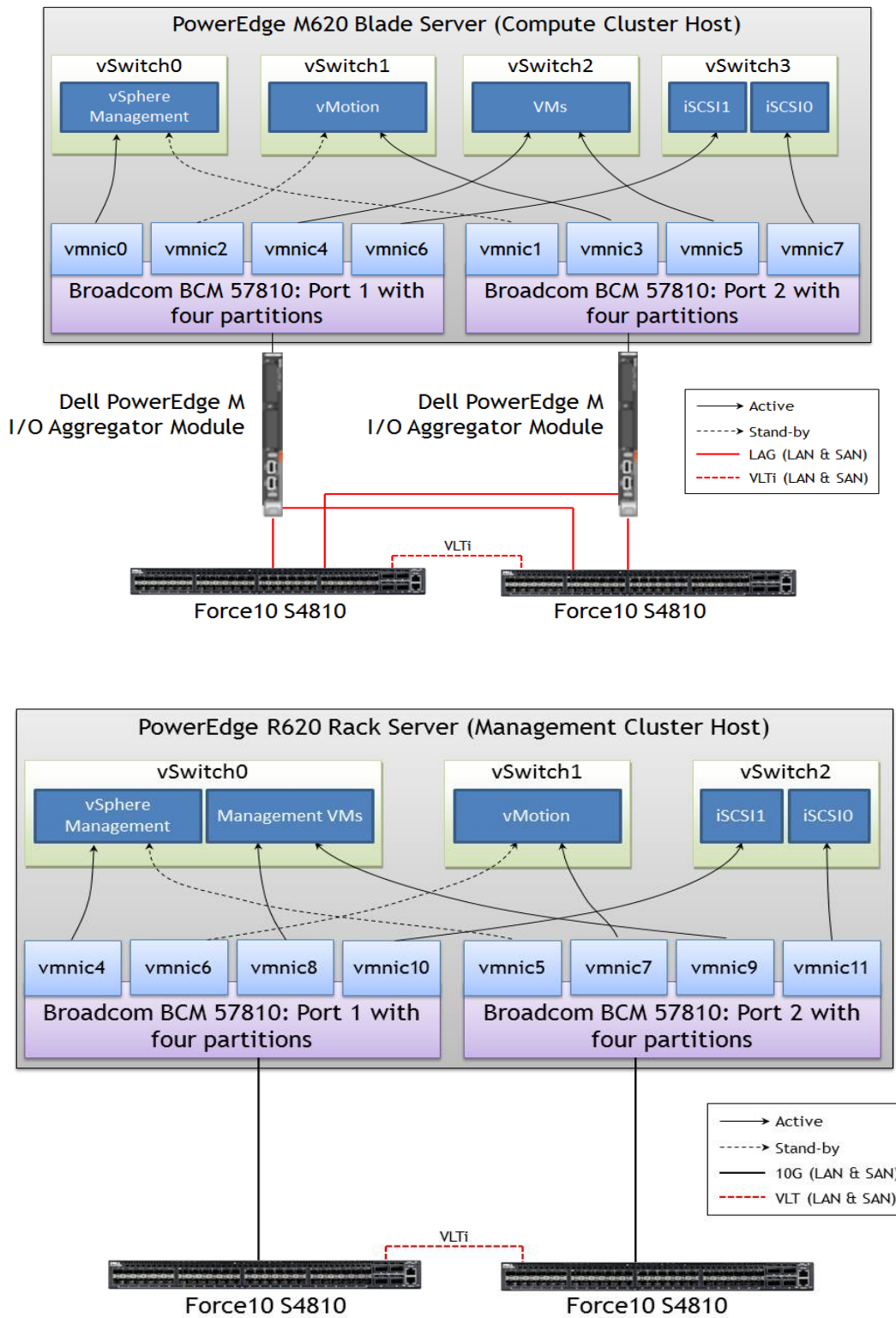
Figure 6: vSwitch and NPAR Configuration for the Hypervisor Hosts
