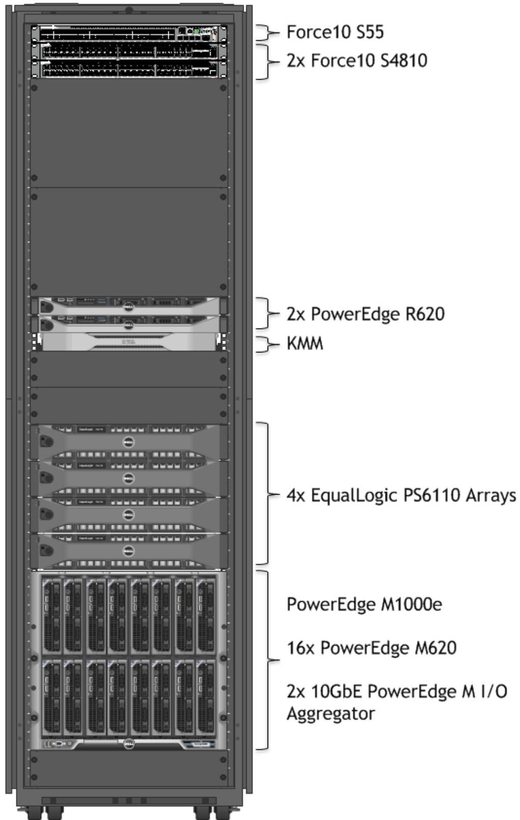
Figure 8: Active System 800v Single Chassis: Rack Overview
