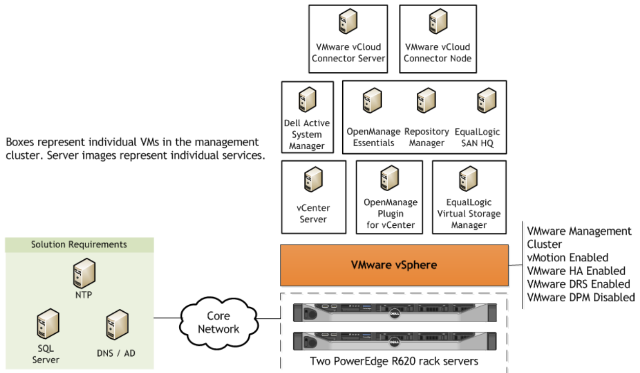
Figure 7: Management Components
