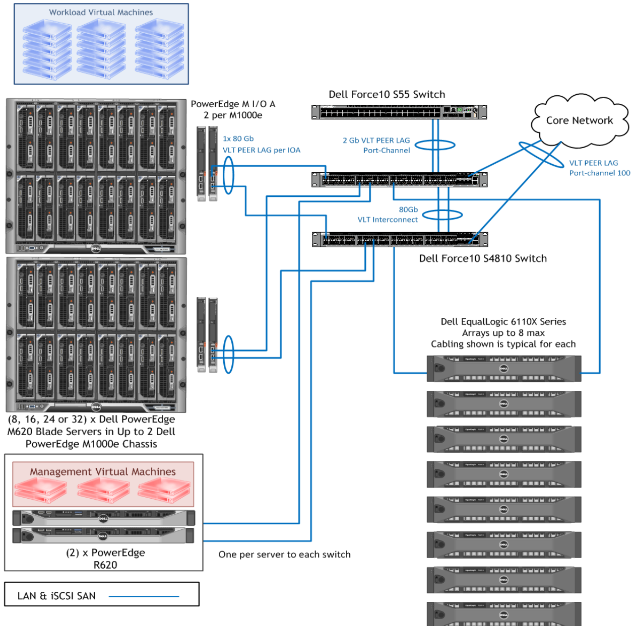
Figure 2: Active System 800v Network Topology (Logical View)
