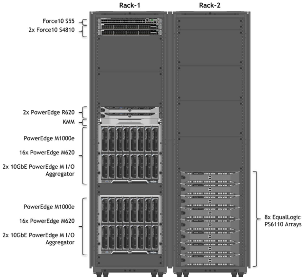
Figure 9: Active System 800v Two Chassis and Maximum Storage: Rack Overview
