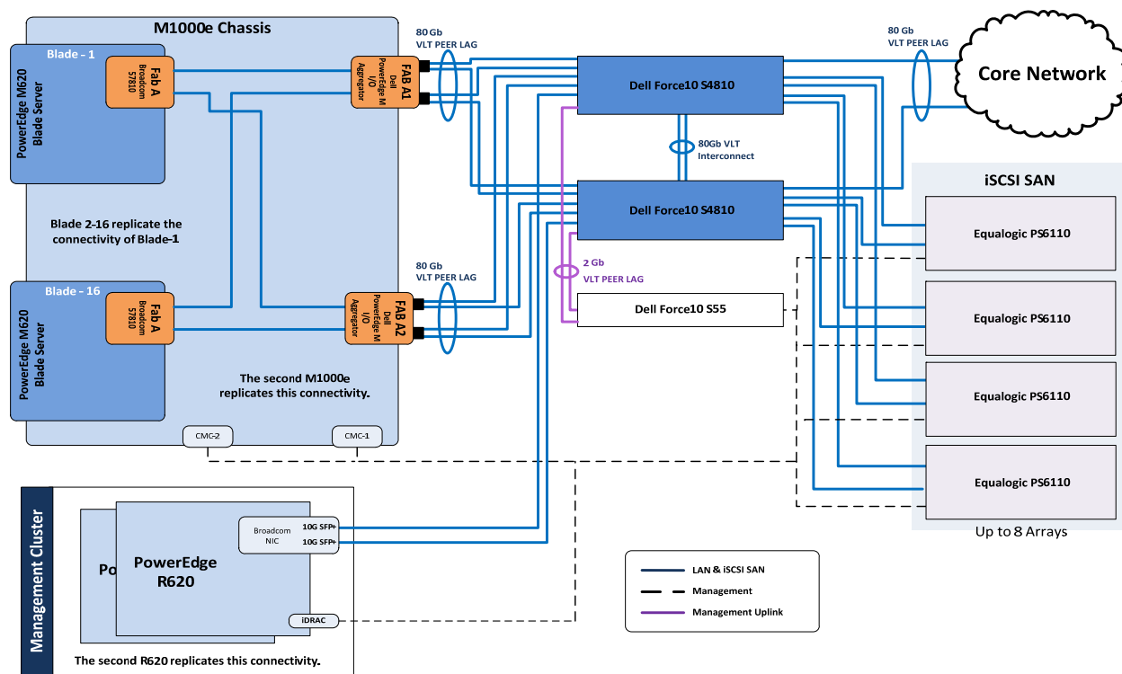
Figure 4: Converged Network Logical Connectivity
